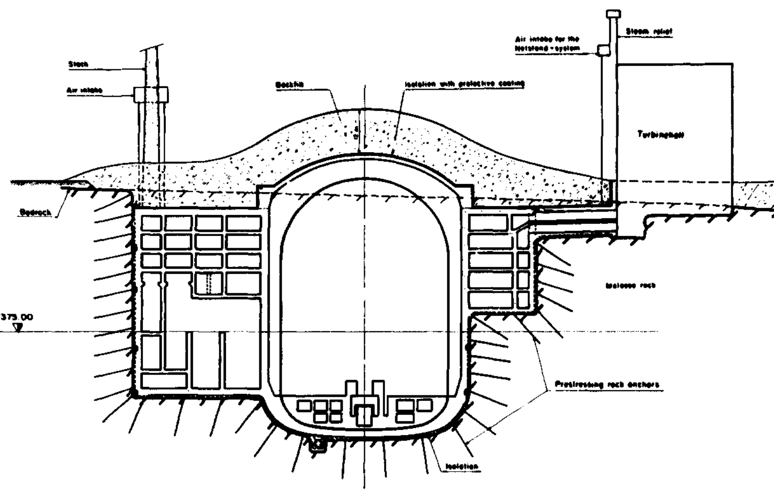
Fig. 6 - 21 Pit siting in rock: vertical section
