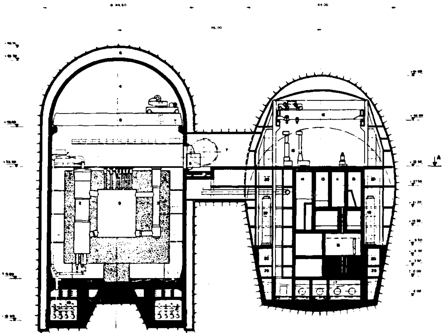
Fig. 6 - 13 HTR plant: vertical section
