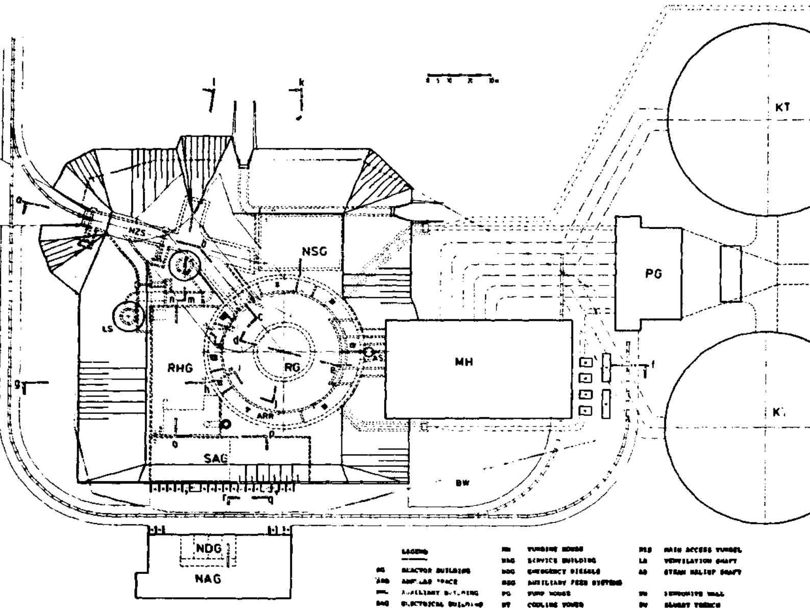
Fig. 5 - 14 BMI-KFA study: totally embedded plant 1
