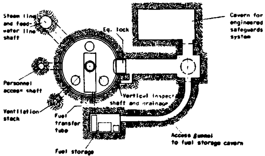
Fig. 6 - 2 Underground PWR - deep below the surface disposition
