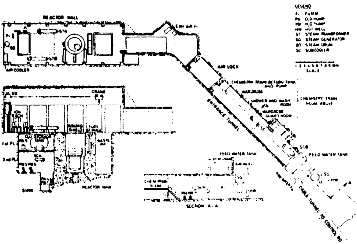
Fig. 1 - 2 Halden plant layout
