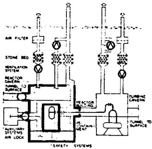
ALTERNATIVE 2 REACTOR WITH COMPLETE CONTAINMENT PLACED TOGETHER WITH AUXILIARY EQUIPMENT IN A CAVERN OPEN TO THE ATMOSPHERE
