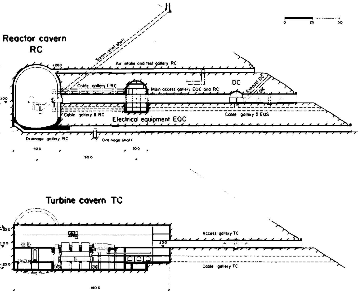
Fig. 6 - 8 EIR rock cavity plant layout: sections
