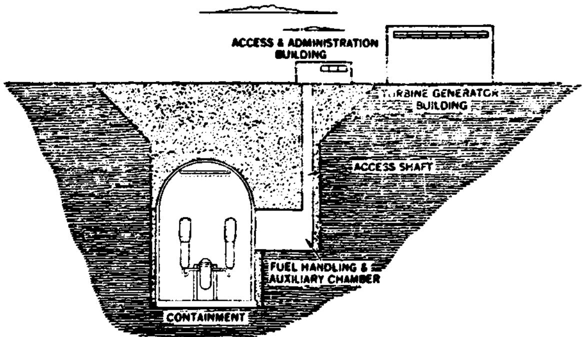
Fig. 4 - 34 Pit siting
