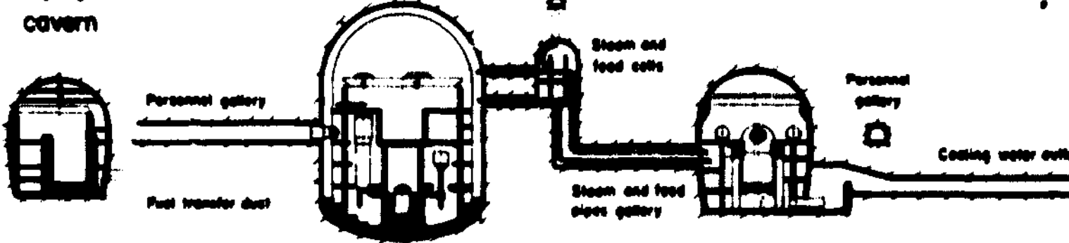
Fig. 6 - 23 Plant totally in rock cavities: sections
