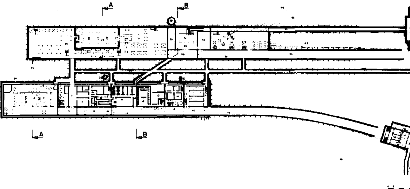
Fig. 6 - 9 BWR in rock cavities: plan
