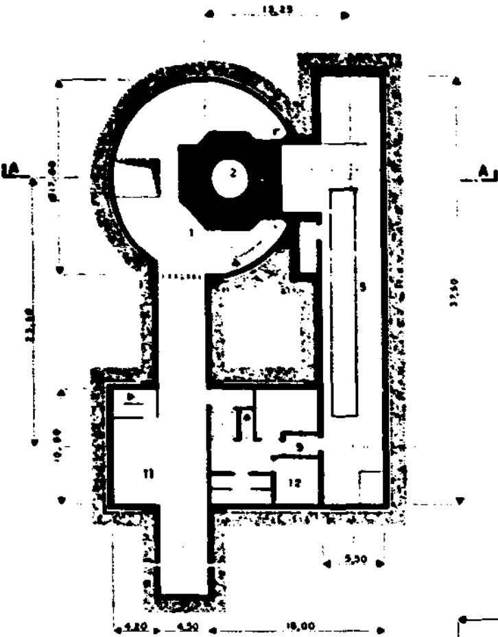
Fig. 1 - 10 Cavern horizontal section (elevation 408.00)
