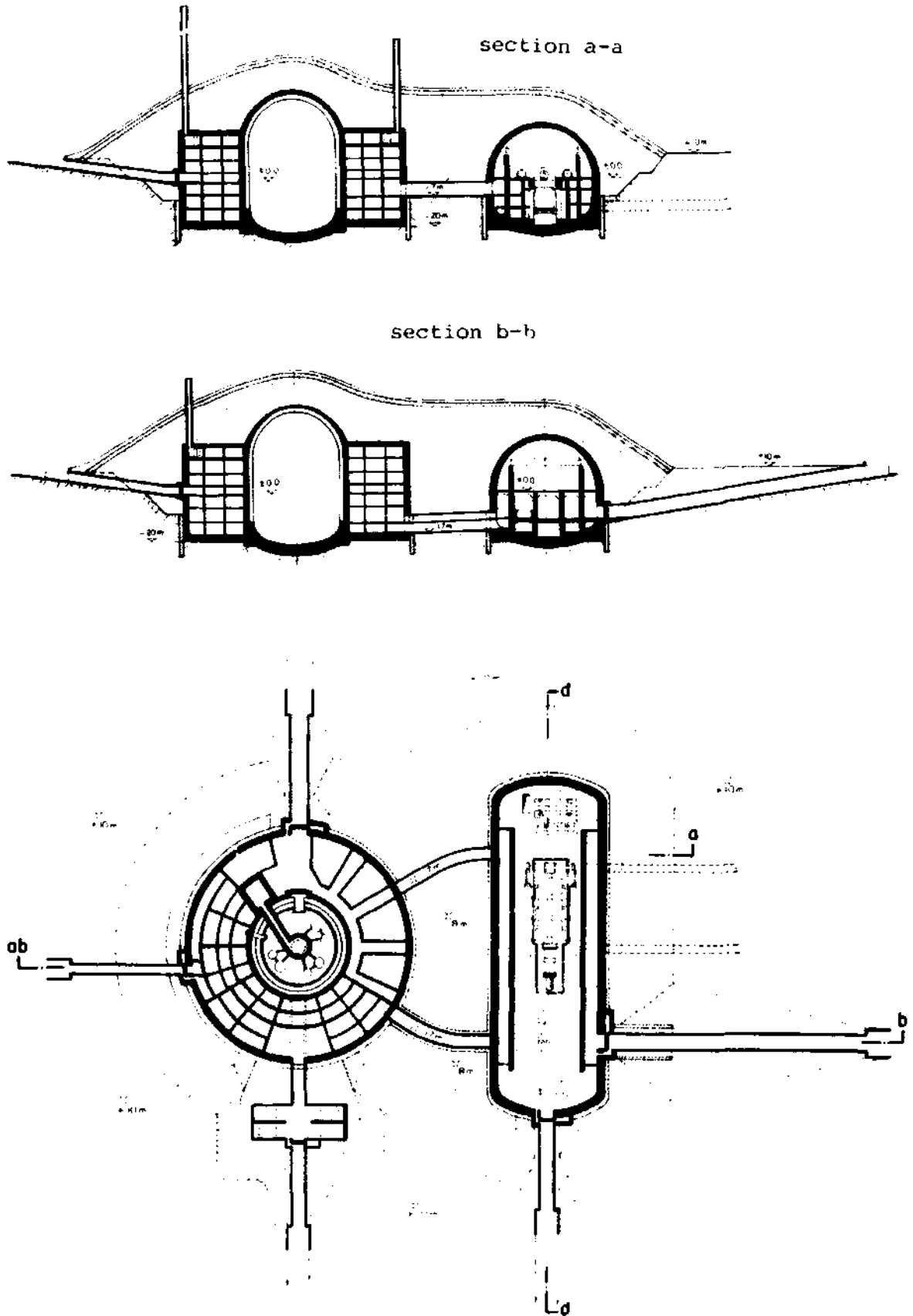
Fig. 6 - 15 EIR pit siting study 1976: plant layout
