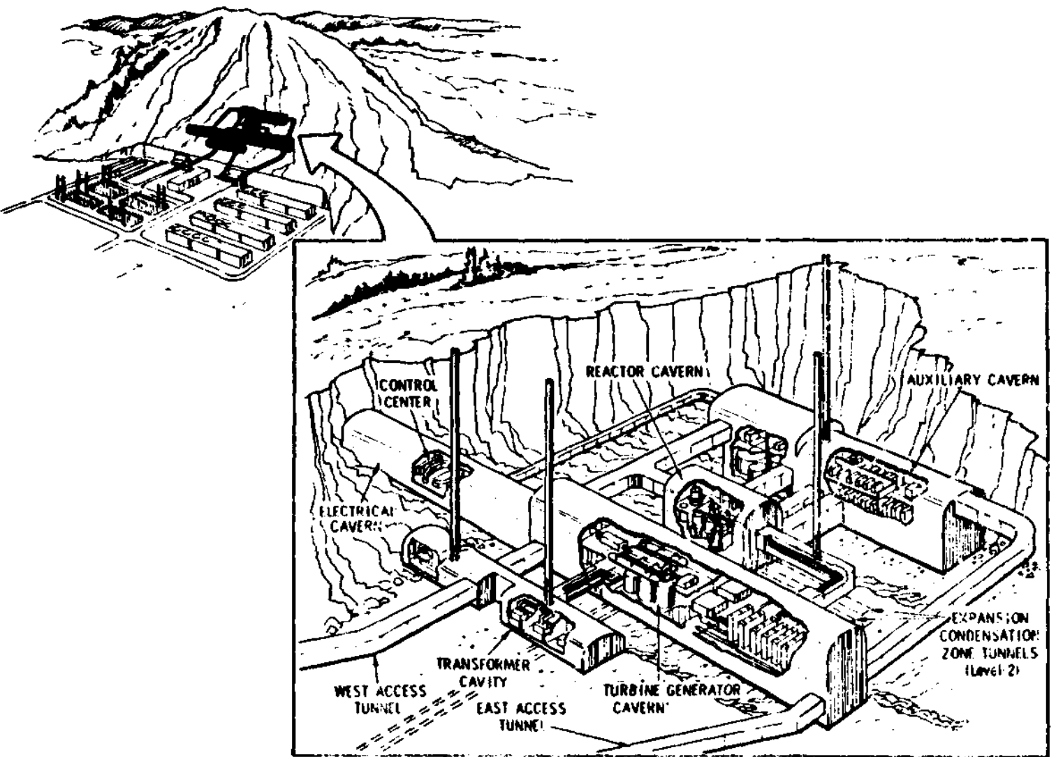
Fig. 4 - 37 Cutaway drawing of the CEC rock cavity plant
